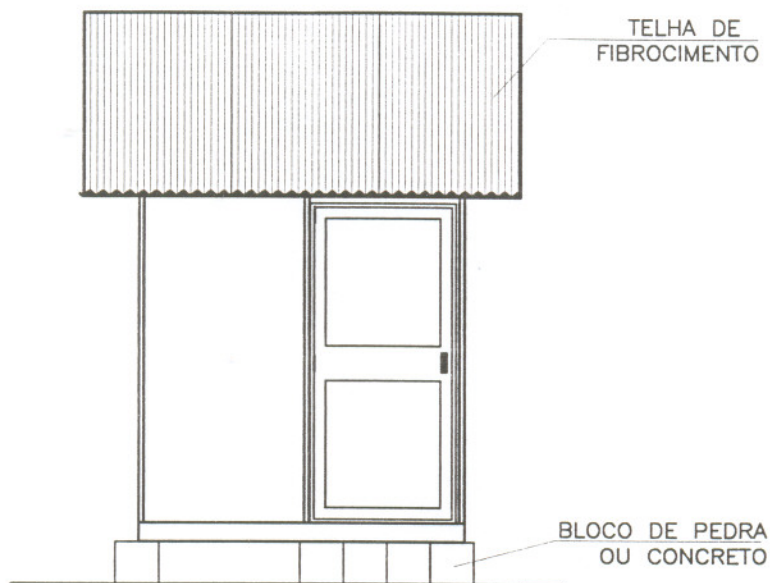
VISTA FRONTAL
